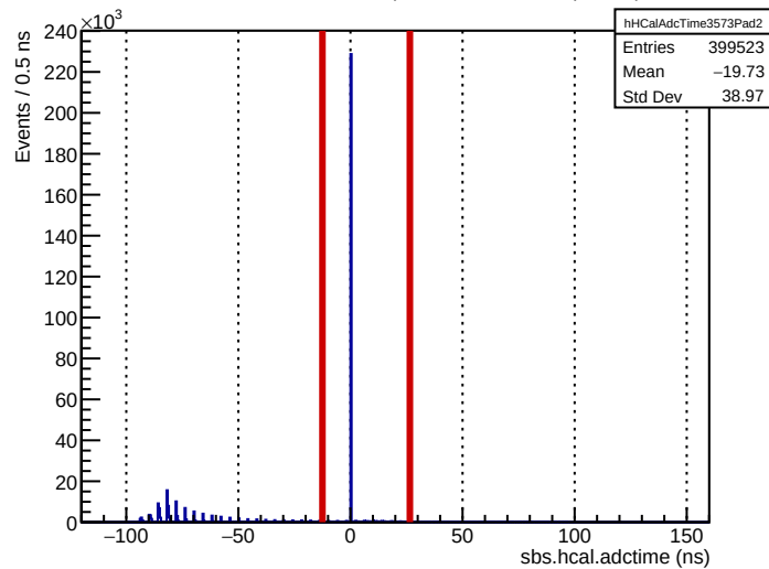
Run 3573: sbs.hcal.adctime (ECal bounds for comparison)
