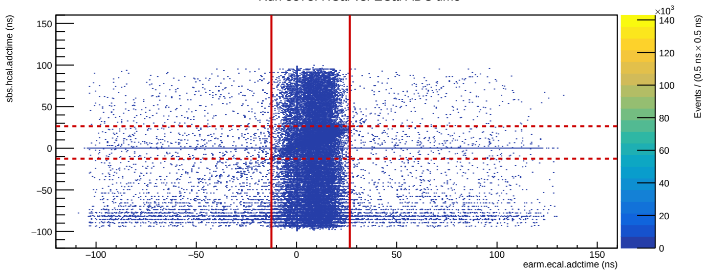
Run 3573: HCal vs. ECal ADC time
