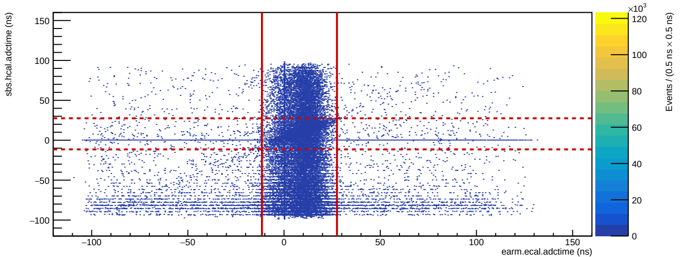
Run 3575: HCal vs. ECal ADC time
