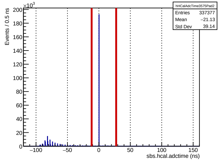
Run 3575: sbs.hcal.adctime (ECal bounds for comparison)
