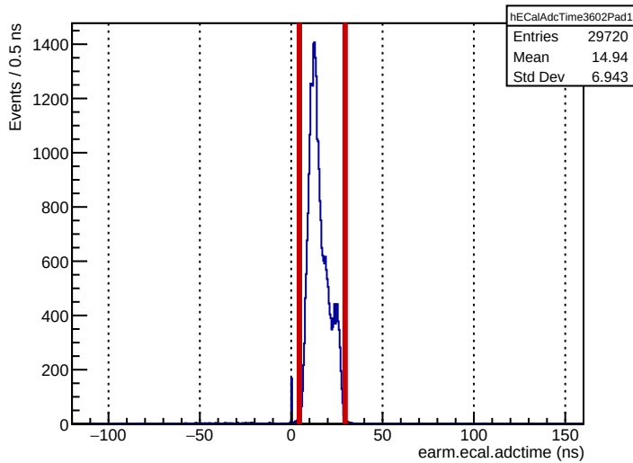
Run 3602: earm.ecal.adctime
