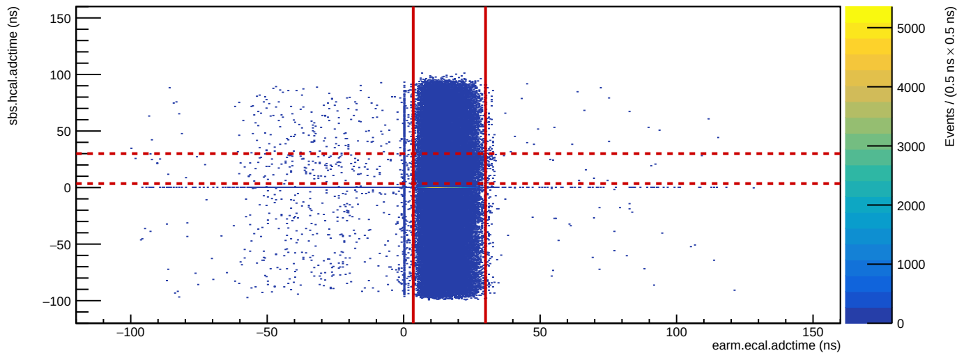
Run 3757: HCal vs. ECal ADC time
