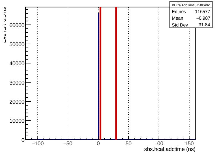
Run 3758: sbs.hcal.adctime (ECal bounds for comparison)
