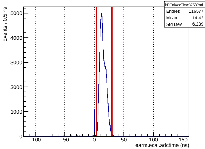
Run 3758: earm.ecal.adctime
