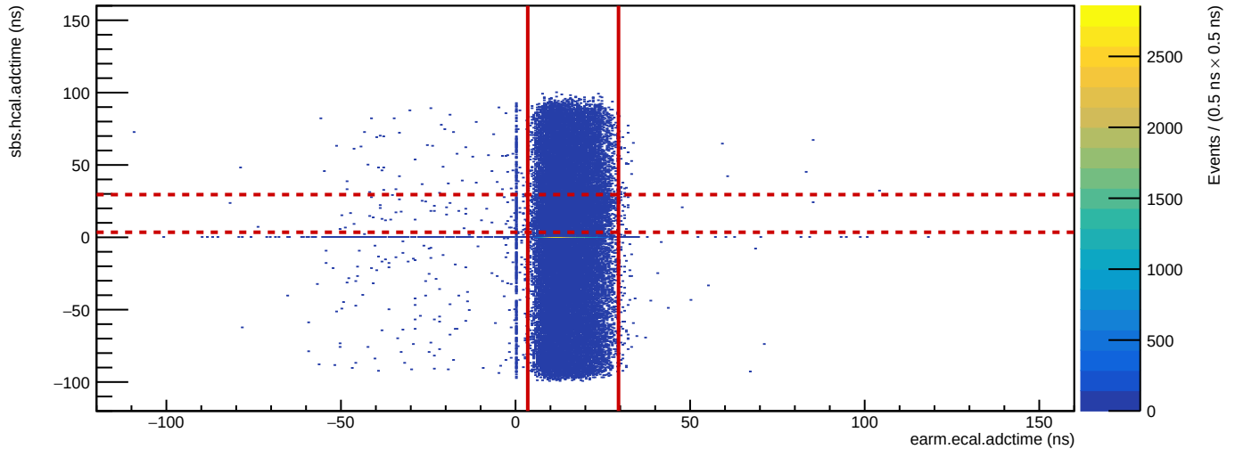
Run 3758: HCal vs. ECal ADC time
