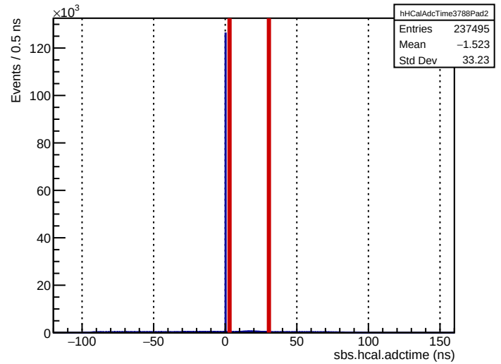
Run 3788: sbs.hcal.adctime (ECal bounds for comparison)
