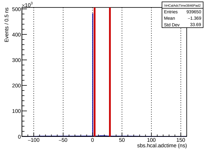
Run 3846: sbs.hcal.adctime (ECal bounds for comparison)
