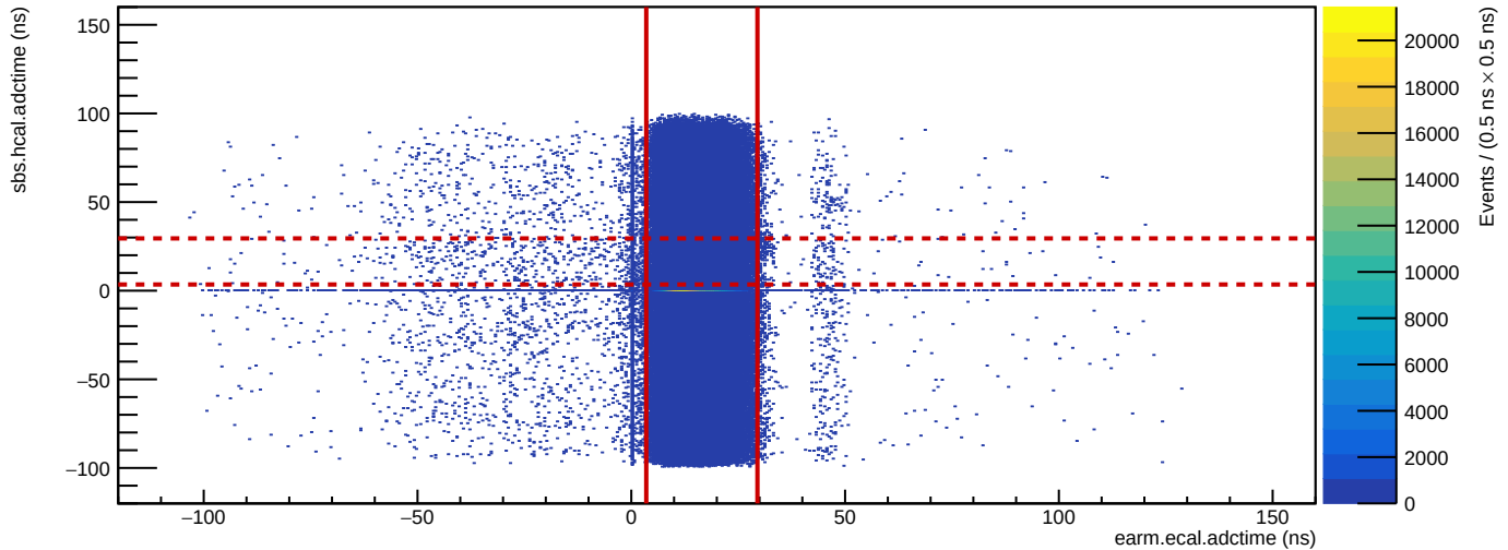
Run 3846: HCal vs. ECal ADC time
