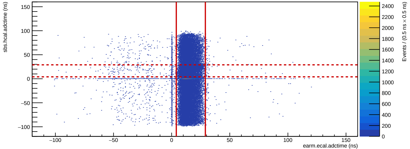
Run 4003: HCal vs. ECal ADC time
