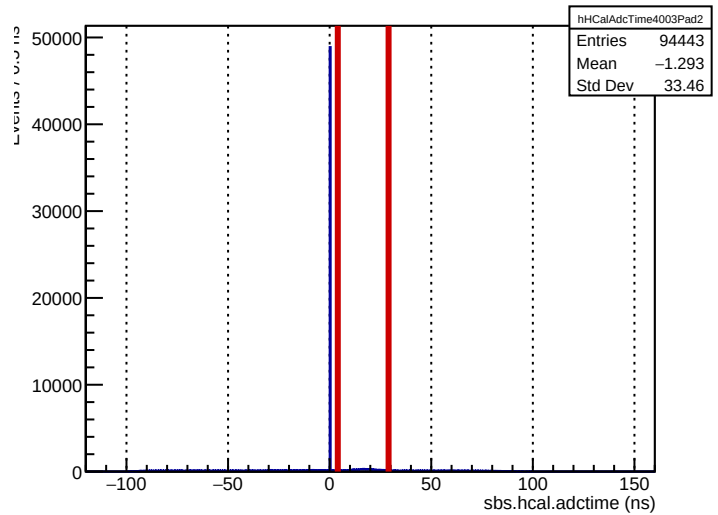
Run 4003: sbs.hcal.adctime (ECal bounds for comparison)
