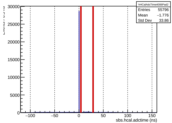
Run 4006: sbs.hcal.adctime (ECal bounds for comparison)
