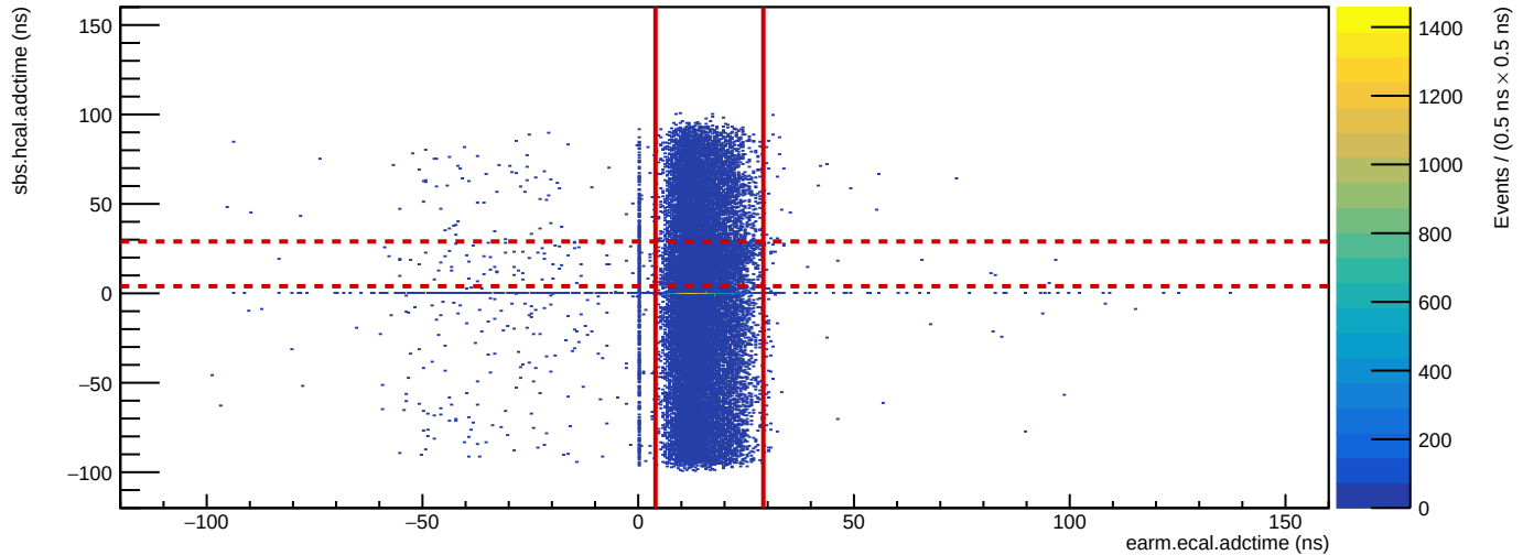
Run 4006: HCal vs. ECal ADC time
