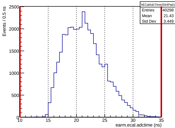
Run 4344: earm.ecal.adctime
