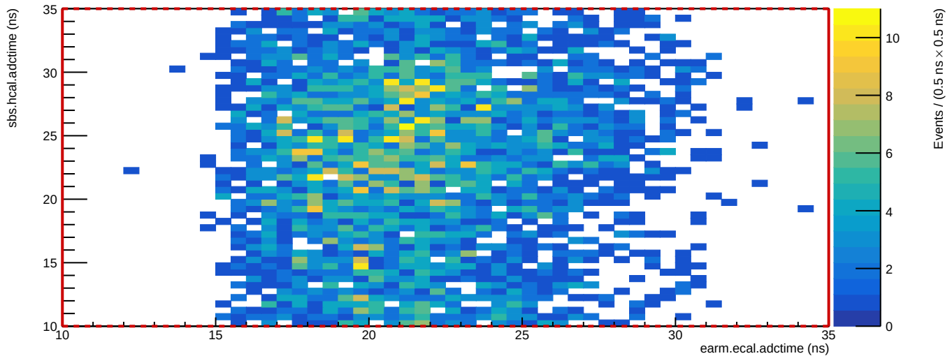
Run 4344: HCal vs. ECal ADC time
