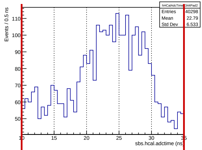
Run 4344: sbs.hcal.adctime (ECal bounds for comparison)
