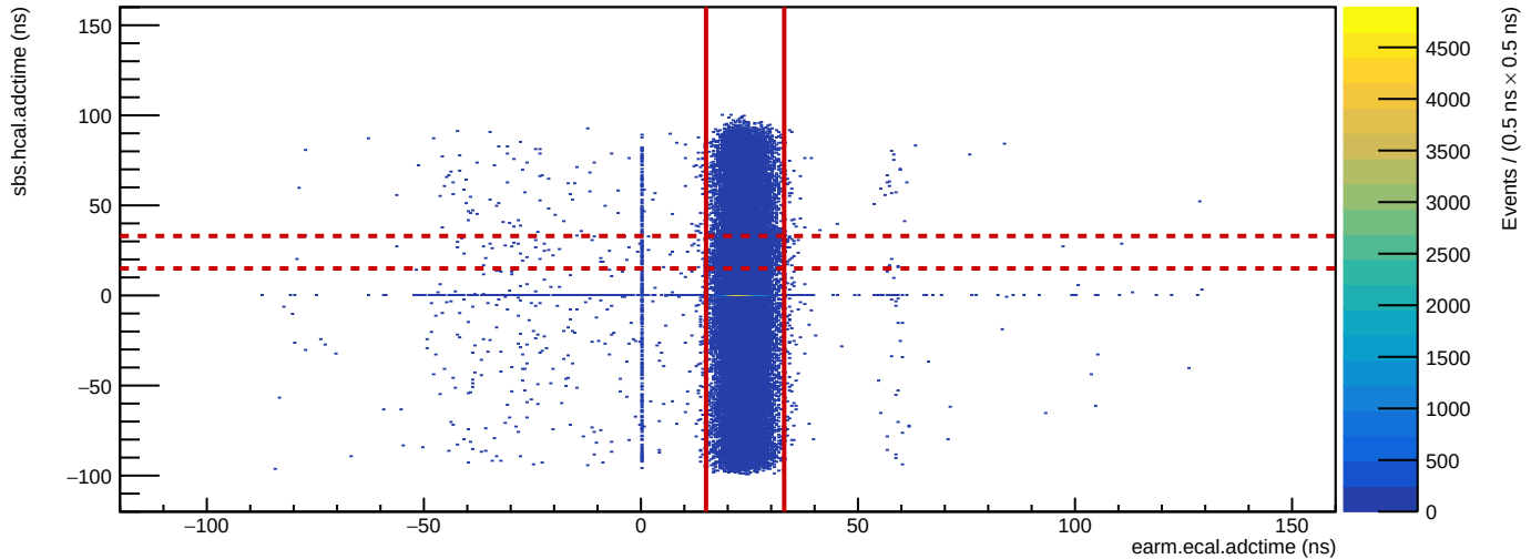
Run 5068: HCal vs. ECal ADC time
