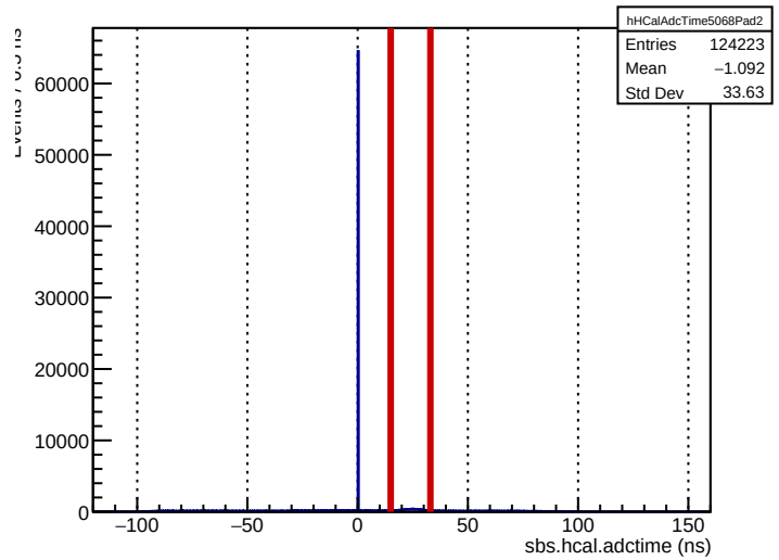
Run 5068: sbs.hcal.adctime (ECal bounds for comparison)
