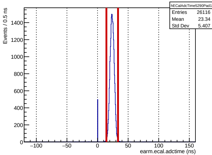
Run 5290: earm.ecal.adctime
