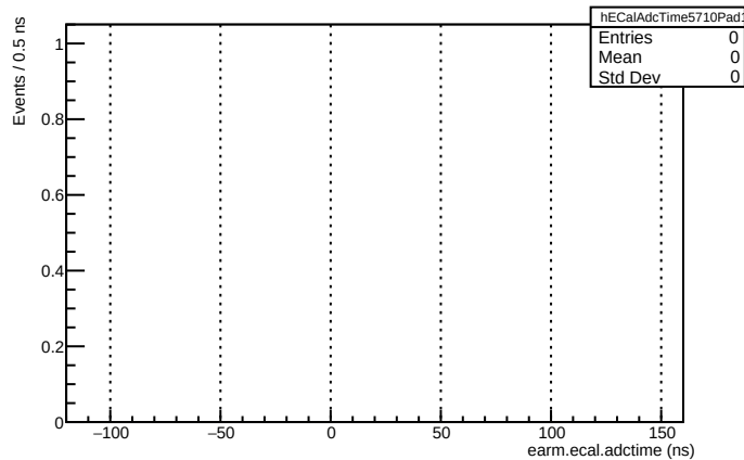
Run 5710: earm.ecal.adctime
