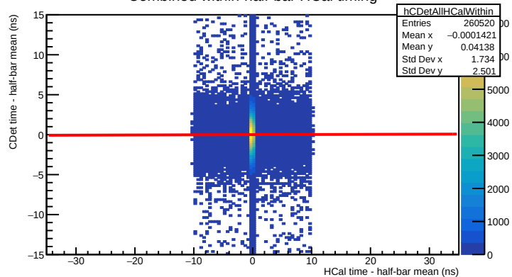
Combined within-half-bar HCal timing
