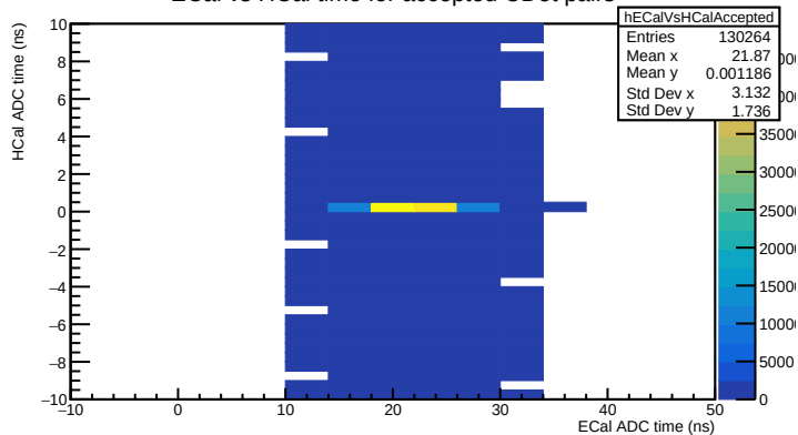
ECal vs HCal time for accepted CDet pairs
