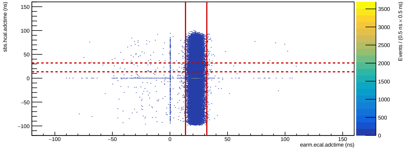
Run 5722: HCal vs. ECal ADC time
