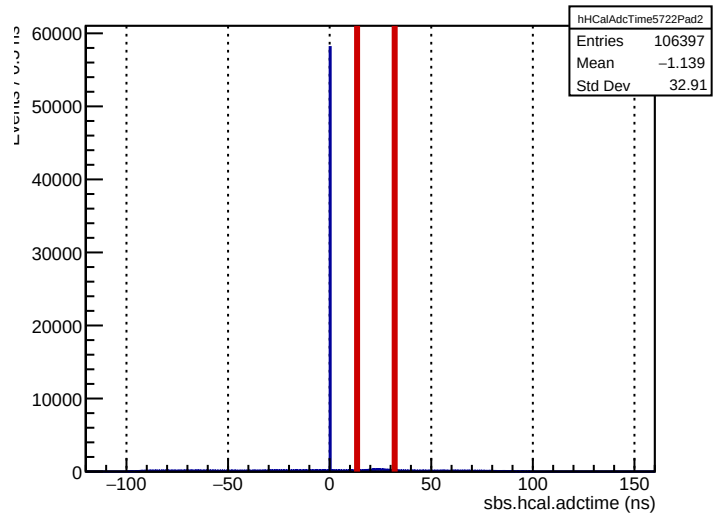
Run 5722: sbs.hcal.adctime (ECal bounds for comparison)
