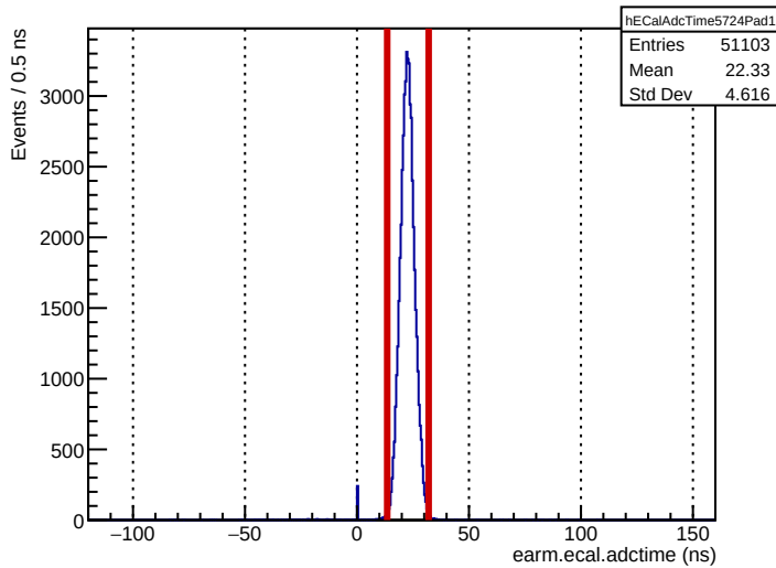
Run 5724: earm.ecal.adctime
