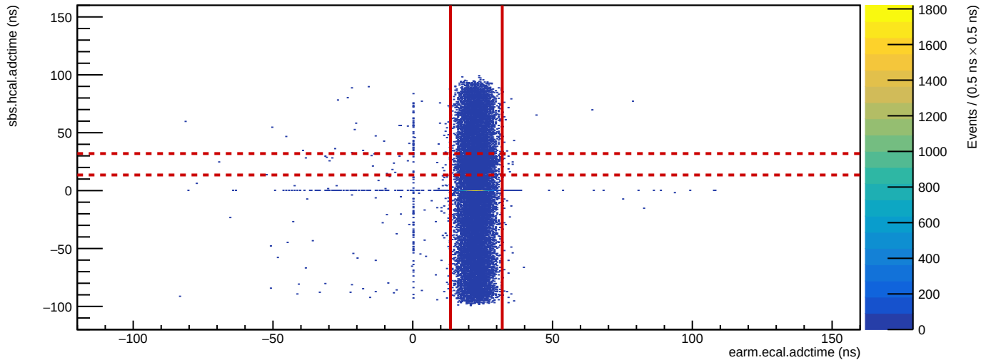
Run 5724: HCal vs. ECal ADC time
