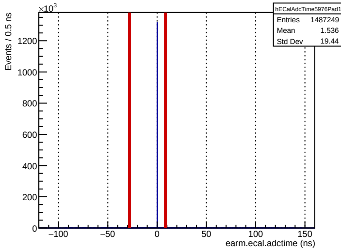
Run 5976: earm.ecal.adctime
