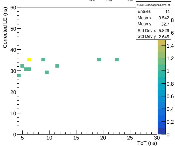
Bar 1L29 diagonal component ( 1 < t_{\text{ECal}} < 18 , |t_{\text{CDet}} - 27 - 0.73 t_{\text{ECal}}| < 3 ns)
