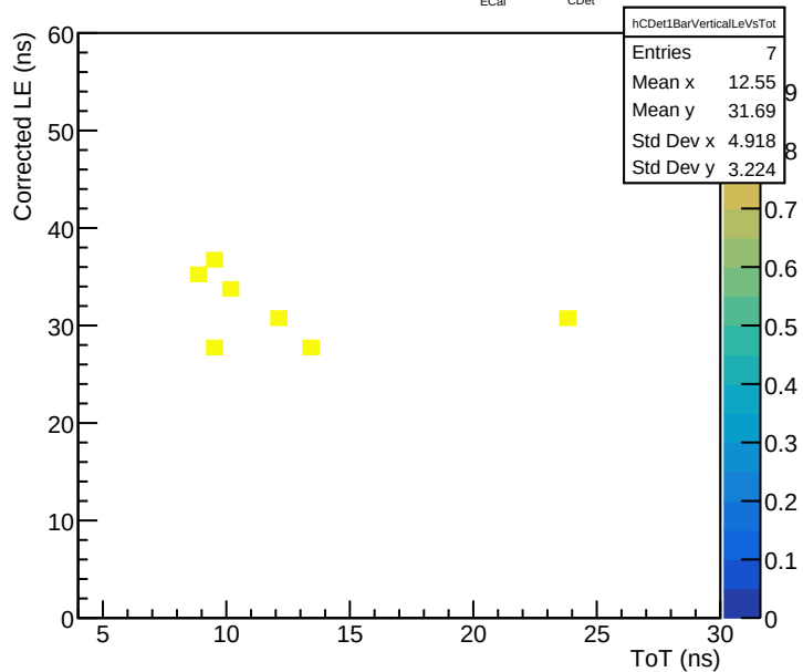
Bar 1L29 vertical ECal-time component ( -3 < t_{\text{ECal}} < 1 , 23 < t_{\text{CDet}} < 40 ns)
