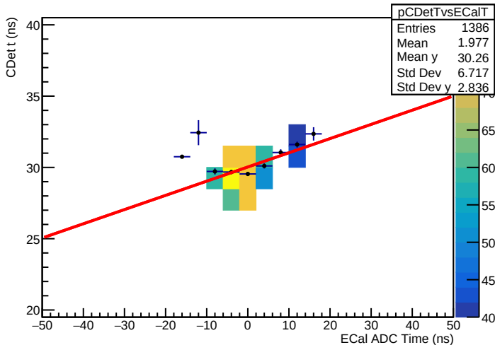
CDet t vs ECal Time
