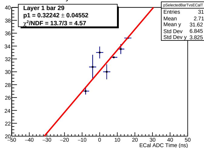
CDet Layer 1 bar 29 t vs ECal Time
