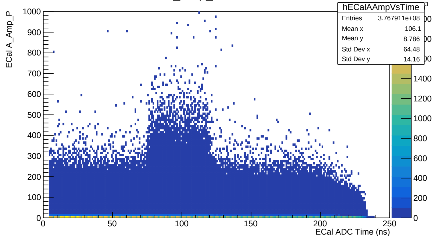
ECal A_Amp_P vs ADC Time
