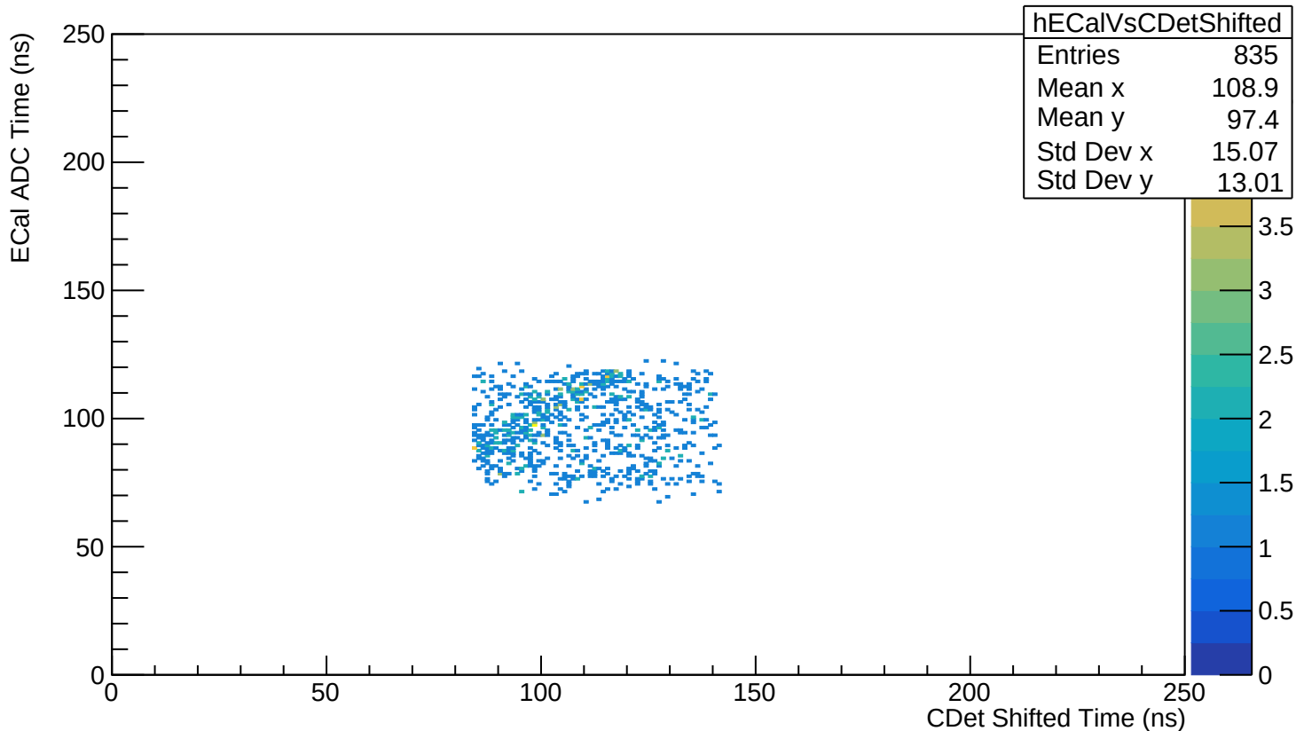
ECal ADC Time vs CDet Shifted Time
