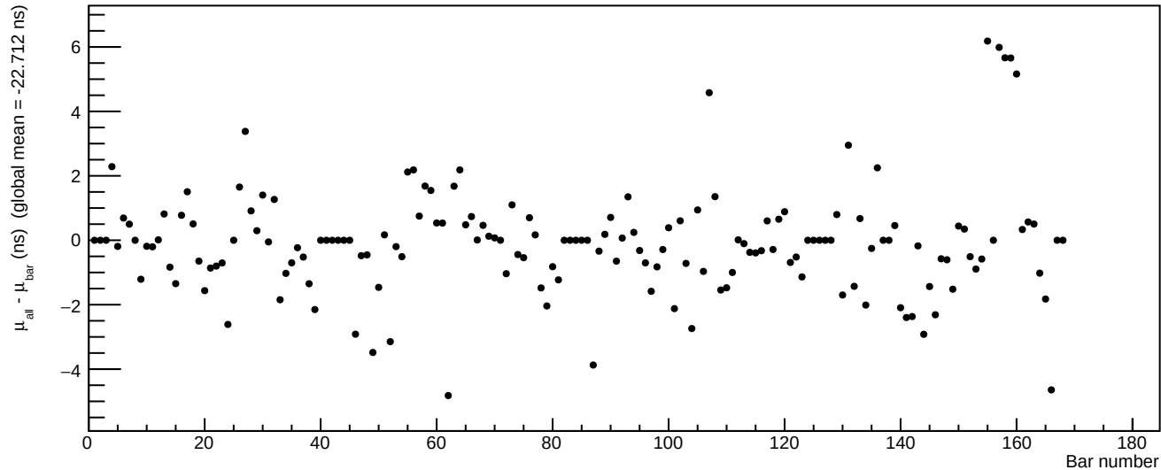
Residual LE offsets vs Bar
