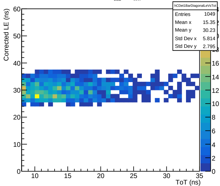
Bar 1L30 diagonal component ( 1 < t_{\text{ECal}} < 18 , |t_{\text{CDet}} - 27 - 0.73 t_{\text{ECal}}| < 3 ns)
