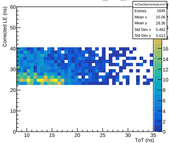
Bar 1L30 vertical ECal-time component ( -3 < t_{\text{ECal}} < 1 , 23 < t_{\text{CDet}} < 40 ns)
