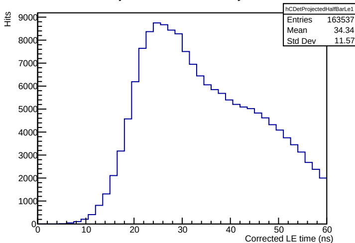
Projected-half-bar hits, Layer 1
