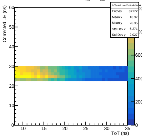
All CDet bars: lower vertical component ( -5 < t_{ECal} < 1 , 23 < t_{CDet} < 30 ns)
