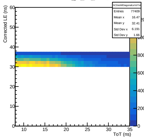
All CDet bars: diagonal component ( t_{ECal} > 1 , t_{CDet} > 30 , |t_{CDet} - 27 - 0.73t_{ECal}| < 3 ns)
