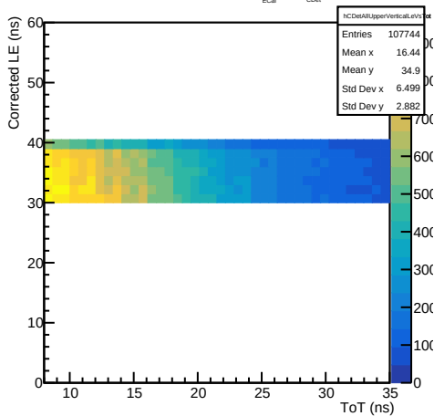
All CDet bars: upper vertical component ( -5 < t_{ECal} < 1 , 30 < t_{CDet} < 40 ns)
