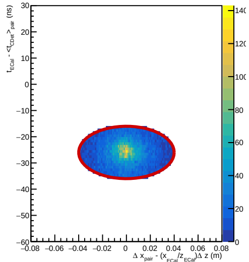
Accepted pairs
