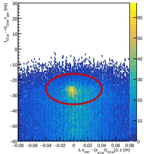
Accepted pairs
