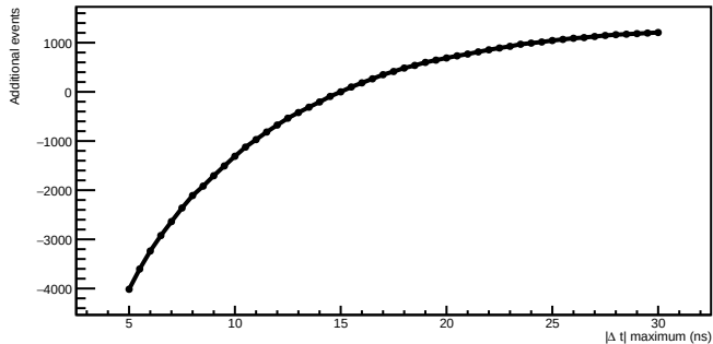
Additional pair events beyond nominal 15 ns gate
