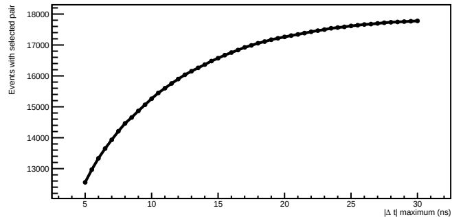
Selected-pair yield versus inter-layer timing gate
