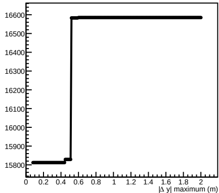
Pair-event yield versus inter-layer y gate
