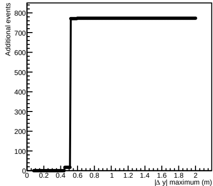
Additional pair events beyond nominal 8 cm gate
