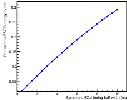
Absolute retention relative to all 3.0--4.5 GeV events
