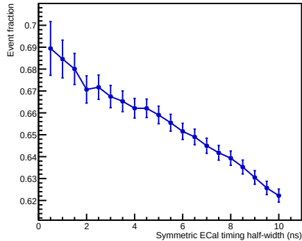
ECal-energy events with \geq 1 selected CDet pair
