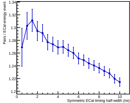
Selected CDet pair yield per ECal-energy event
