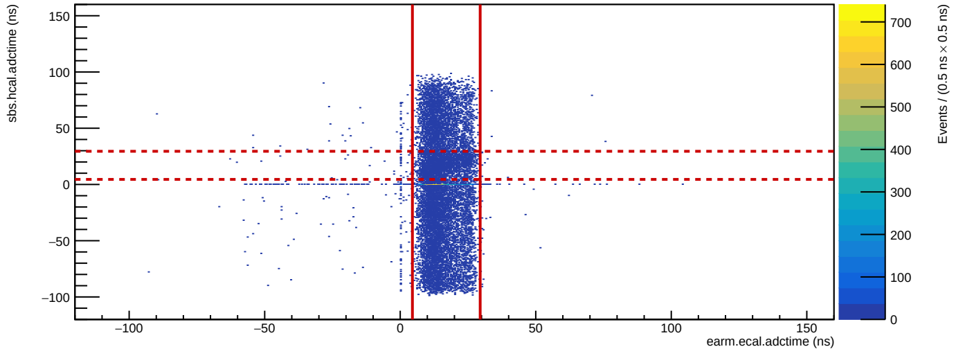
Run 3603: HCal vs. ECal ADC time
