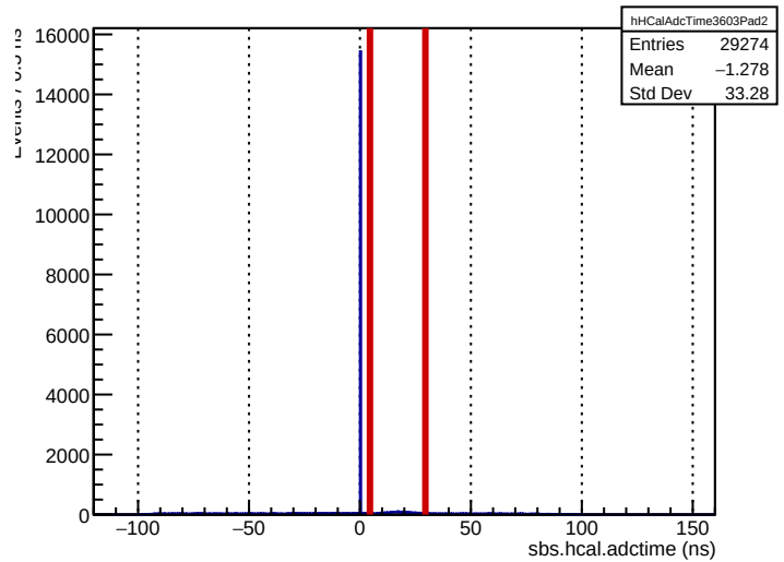
Run 3603: sbs.hcal.adctime (ECal bounds for comparison)
