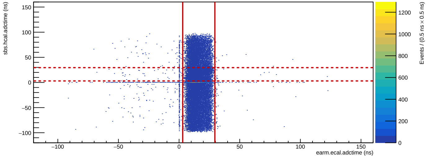
Run 3648: HCal vs. ECal ADC time
