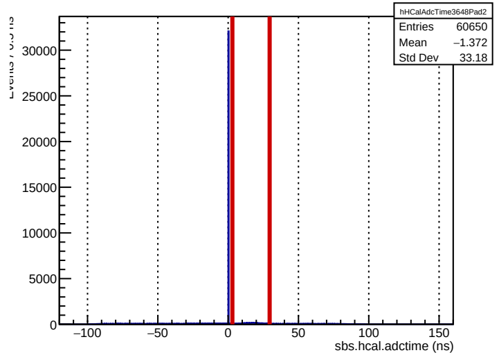
Run 3648: sbs.hcal.adctime (ECal bounds for comparison)
