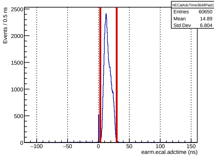
Run 3648: earm.ecal.adctime
