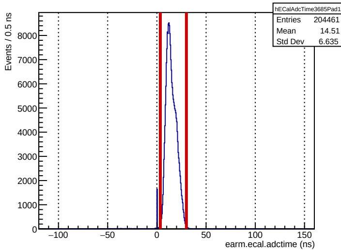
Run 3685: earm.ecal.adctime
