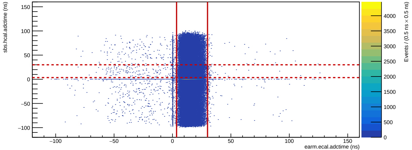
Run 3685: HCal vs. ECal ADC time
