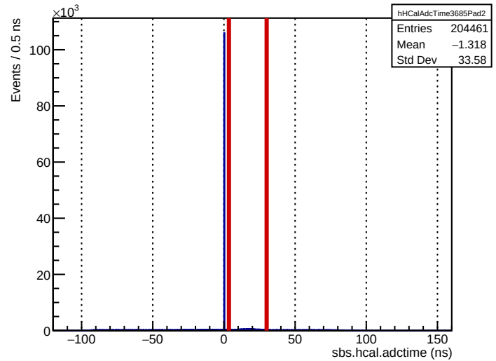
Run 3685: sbs.hcal.adctime (ECal bounds for comparison)
