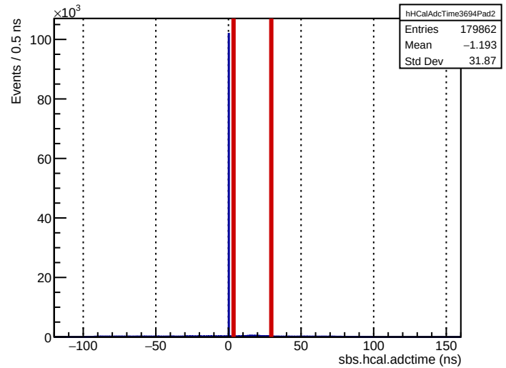
Run 3694: sbs.hcal.adctime (ECal bounds for comparison)
