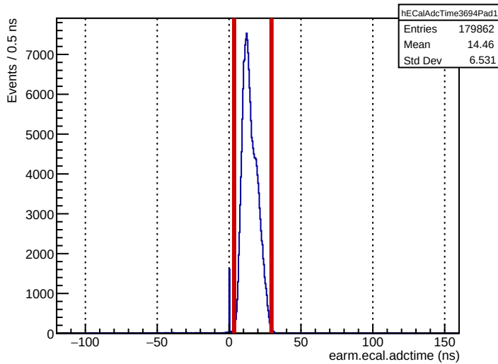
Run 3694: earm.ecal.adctime
