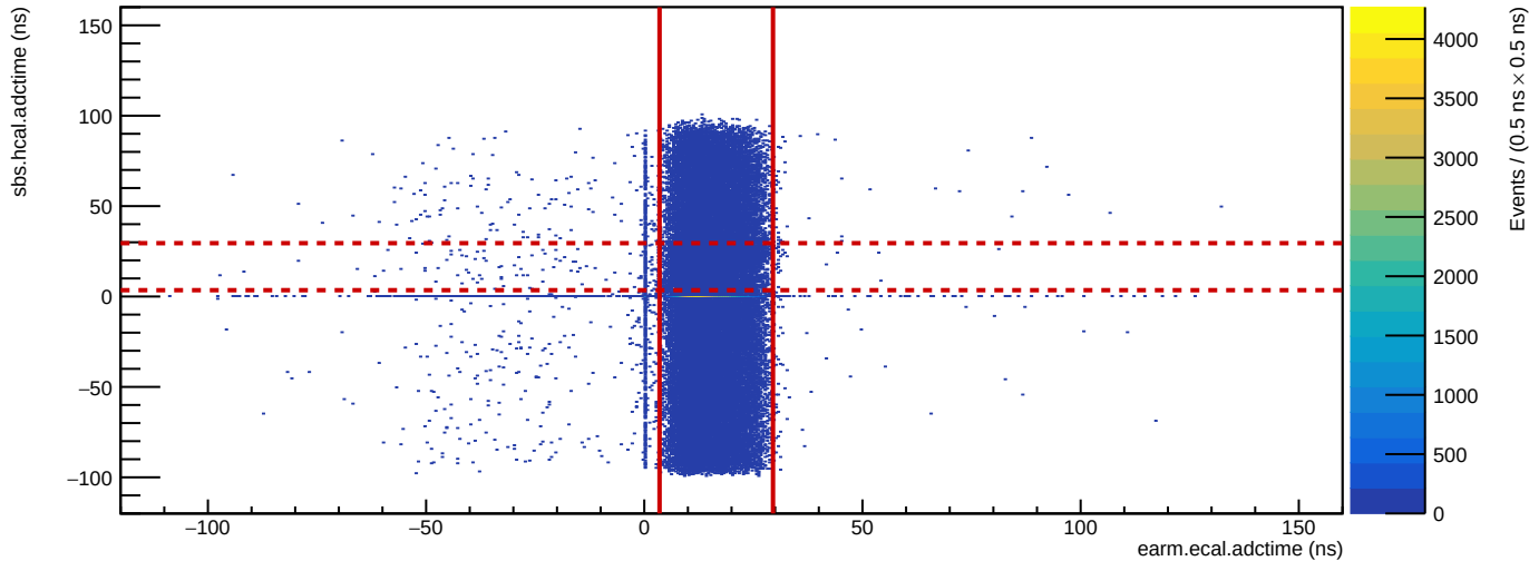
Run 3694: HCal vs. ECal ADC time
