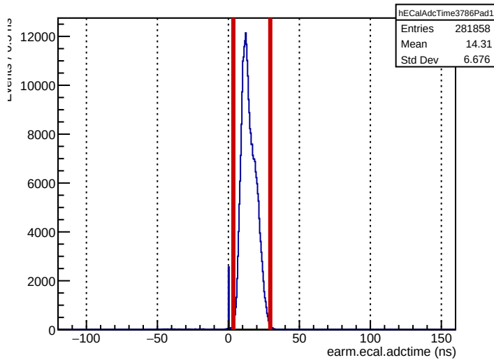
Run 3786: earm.ecal.adctime
