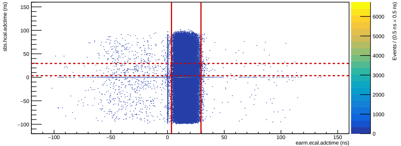
Run 3786: HCal vs. ECal ADC time
