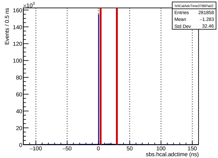
Run 3786: sbs.hcal.adctime (ECal bounds for comparison)
