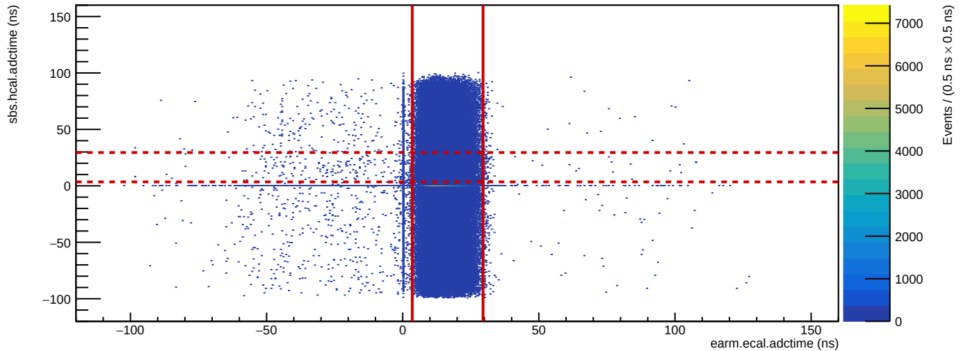
Run 3844: HCal vs. ECal ADC time
