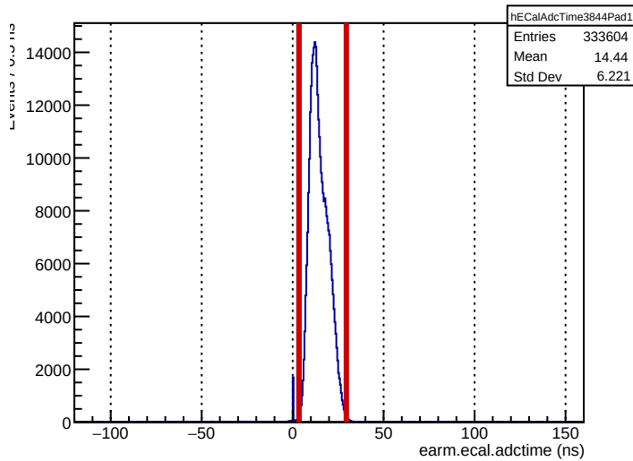
Run 3844: earm.ecal.adctime
