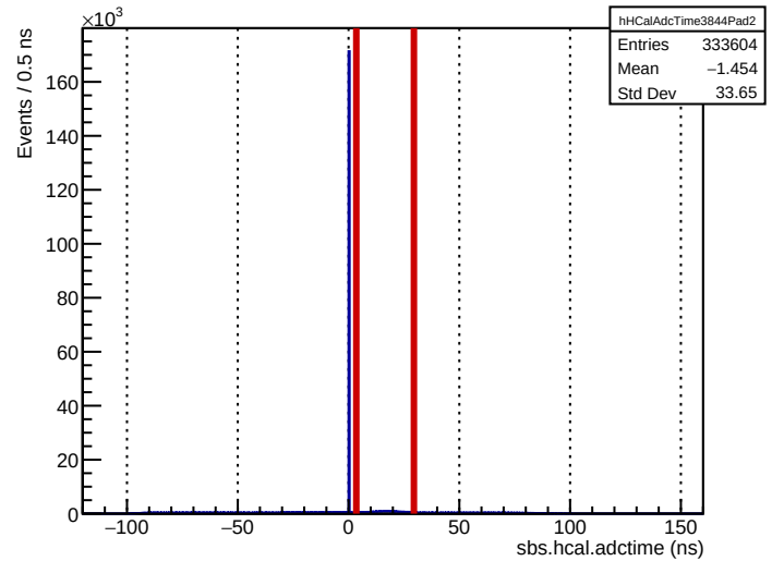
Run 3844: sbs.hcal.adctime (ECal bounds for comparison)
