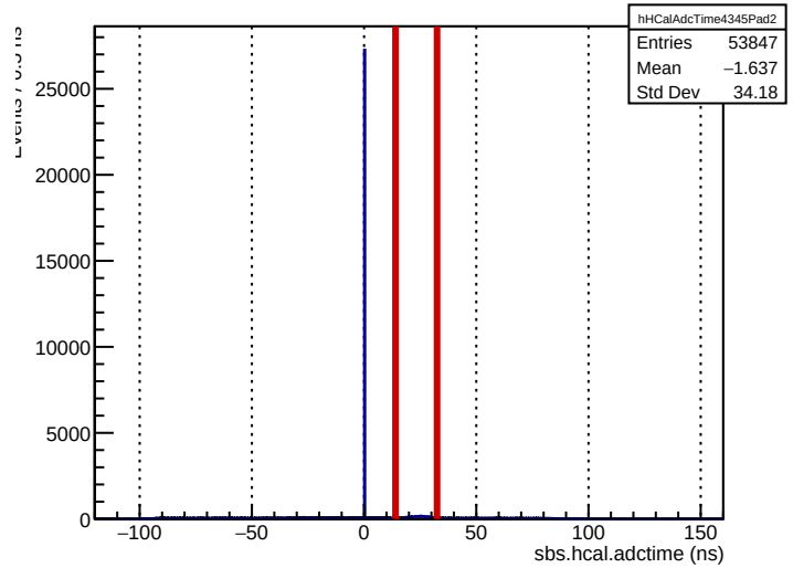
Run 4345: sbs.hcal.adctime (ECal bounds for comparison)
