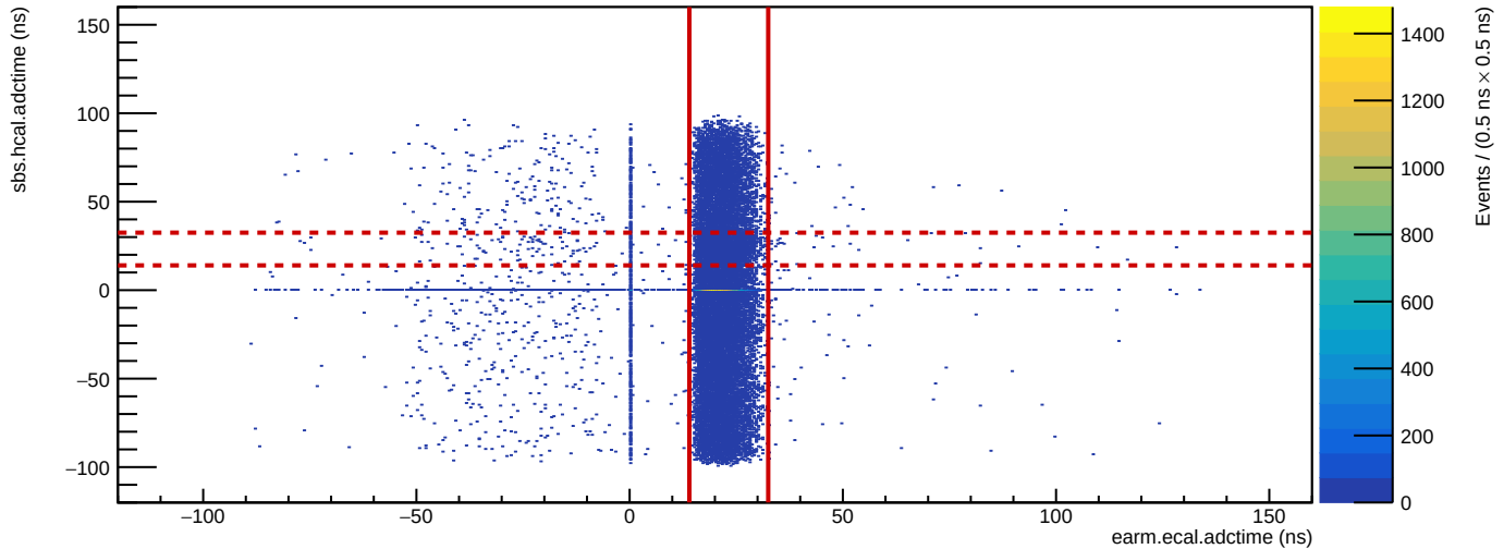
Run 4345: HCal vs. ECal ADC time
