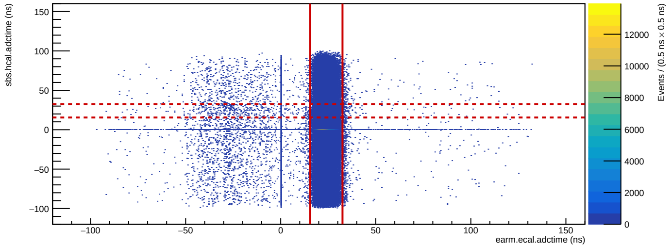
Run 4400: HCal vs. ECal ADC time
