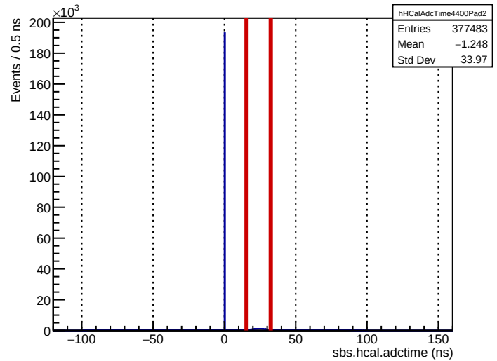
Run 4400: sbs.hcal.adctime (ECal bounds for comparison)
