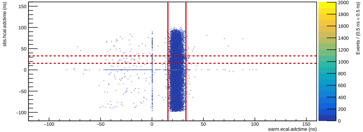
Run 4722: HCal vs. ECal ADC time
