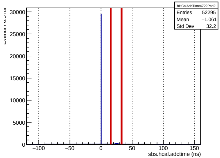
Run 4722: sbs.hcal.adctime (ECal bounds for comparison)
