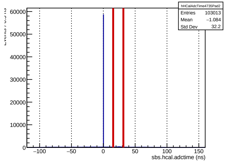
Run 4735: sbs.hcal.adctime (ECal bounds for comparison)
