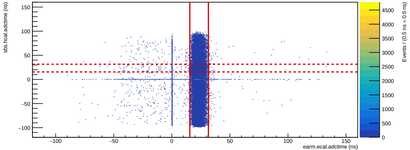
Run 4735: HCal vs. ECal ADC time
