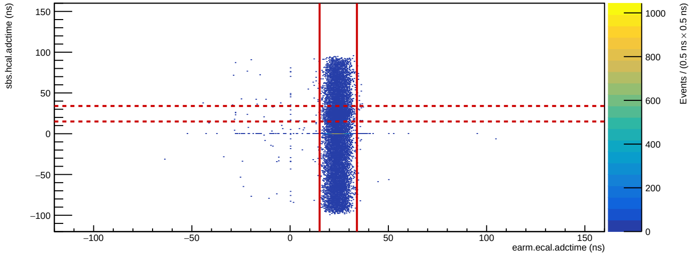
Run 4929: HCal vs. ECal ADC time
