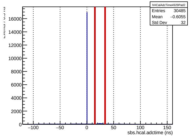
Run 4929: sbs.hcal.adctime (ECal bounds for comparison)
