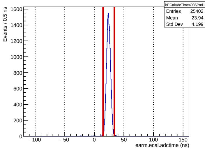
Run 4985: earm.ecal.adctime
