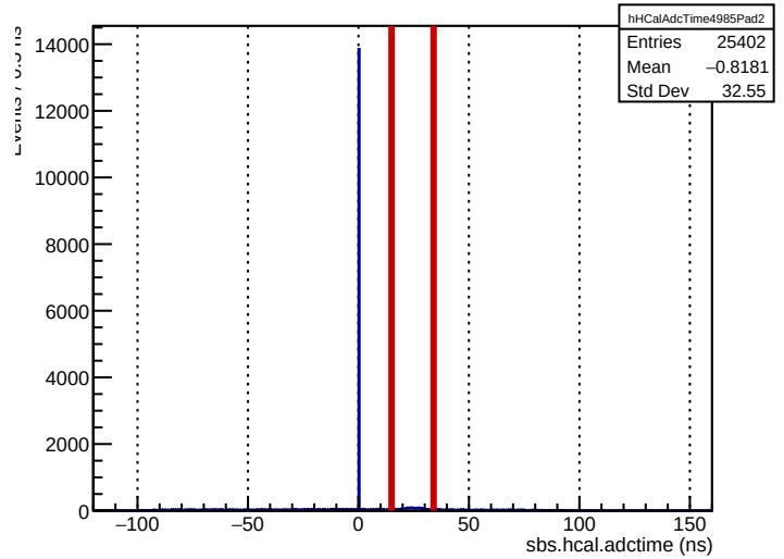
Run 4985: sbs.hcal.adctime (ECal bounds for comparison)
