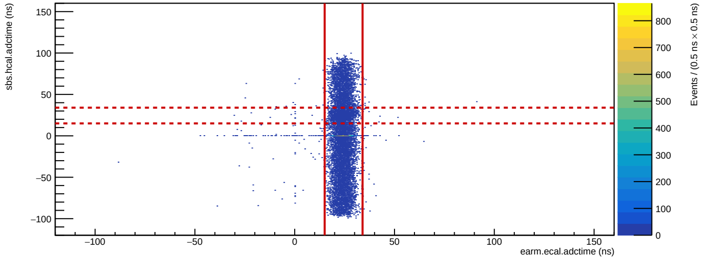
Run 4985: HCal vs. ECal ADC time
