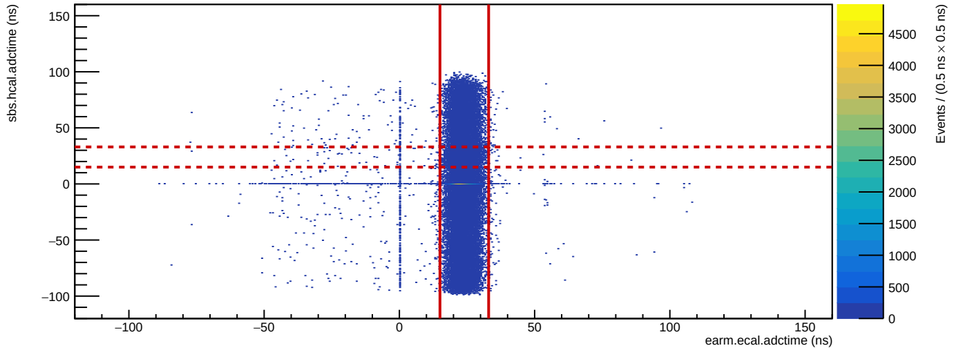
Run 5066: HCal vs. ECal ADC time
