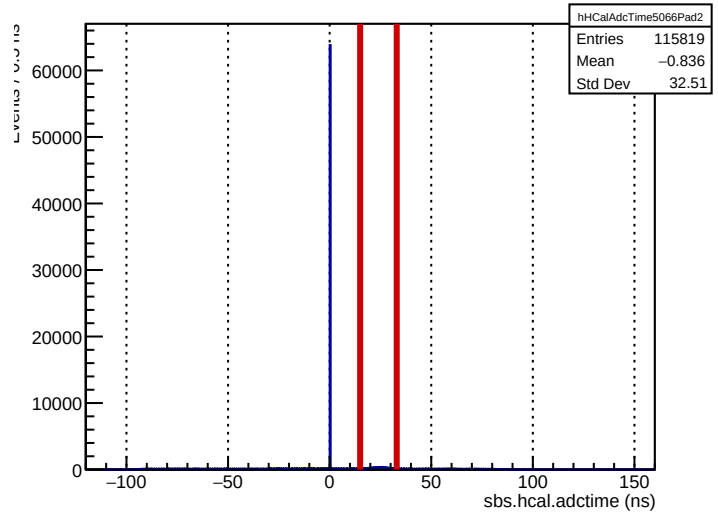
Run 5066: sbs.hcal.adctime (ECal bounds for comparison)
