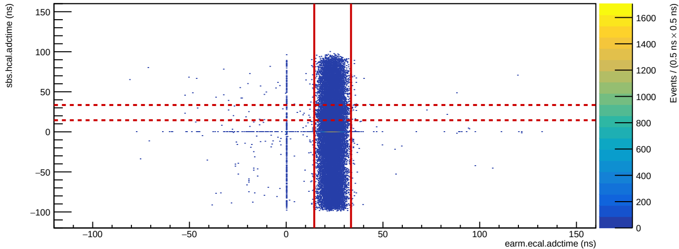
Run 5292: HCal vs. ECal ADC time
