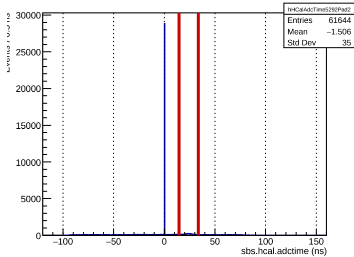
Run 5292: sbs.hcal.adctime (ECal bounds for comparison)
