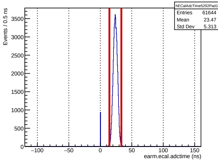
Run 5292: earm.ecal.adctime
