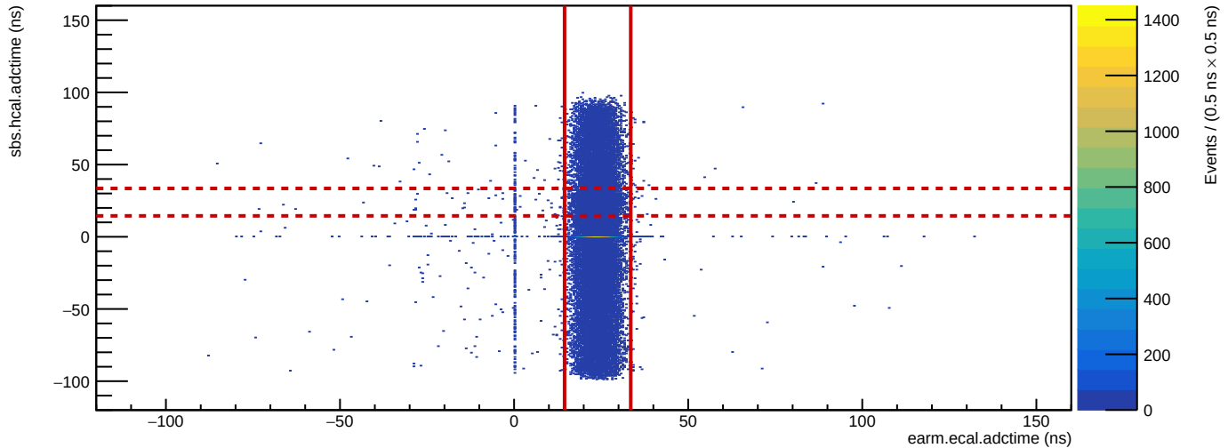
Run 5294: HCal vs. ECal ADC time
