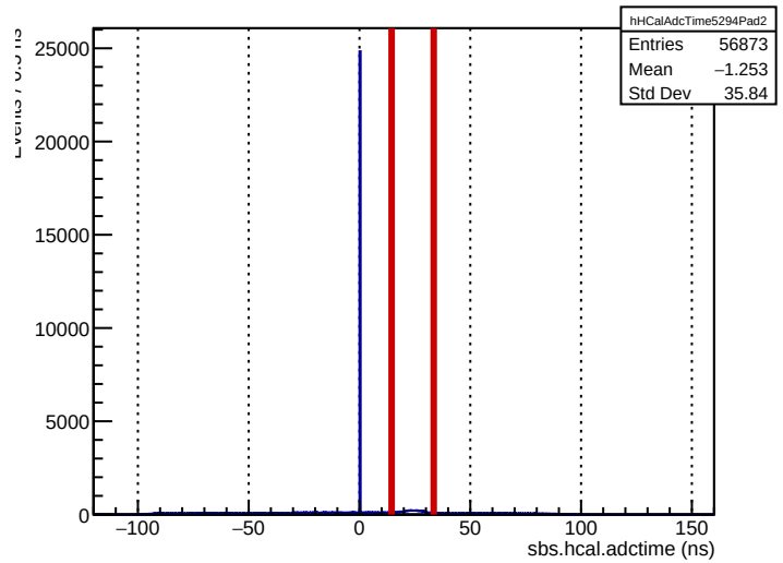
Run 5294: sbs.hcal.adctime (ECal bounds for comparison)
