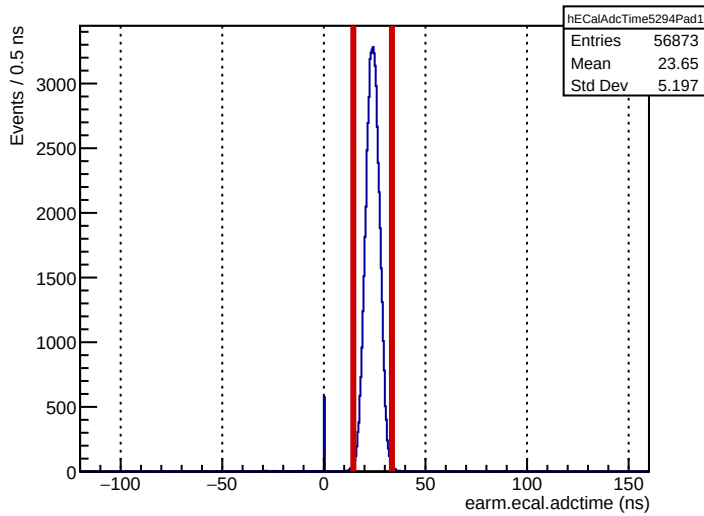
Run 5294: earm.ecal.adctime
