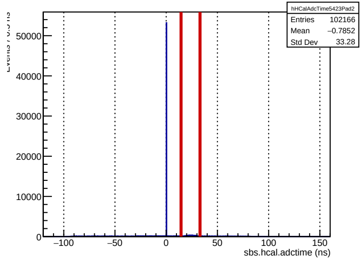
Run 5423: sbs.hcal.adctime (ECal bounds for comparison)
