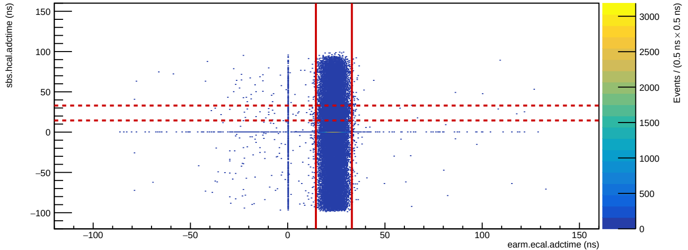
Run 5423: HCal vs. ECal ADC time
