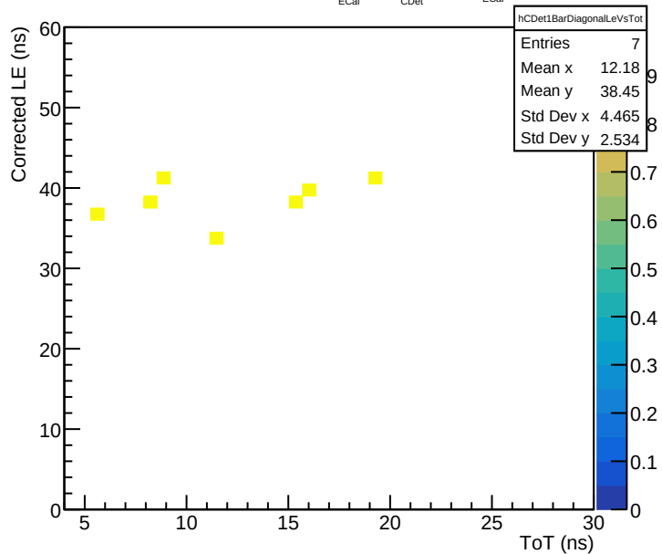
Bar 1L30 diagonal component ( 1 < t_{\text{ECal}} < 18 , |t_{\text{CDet}} - 27 - 0.73t_{\text{ECal}}| < 3 ns)
