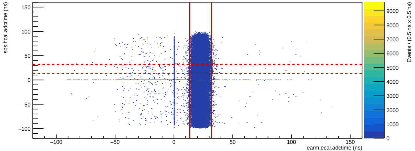
Run 5723: HCal vs. ECal ADC time
