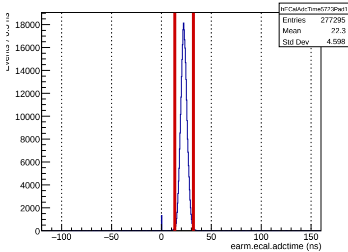
Run 5723: earm.ecal.adctime
