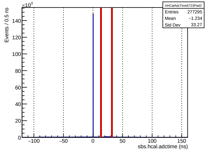
Run 5723: sbs.hcal.adctime (ECal bounds for comparison)
