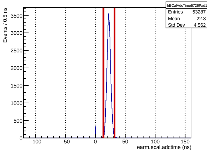
Run 5726: earm.ecal.adctime
