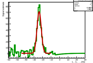
Background-subtracted, logical pixel ID 489
