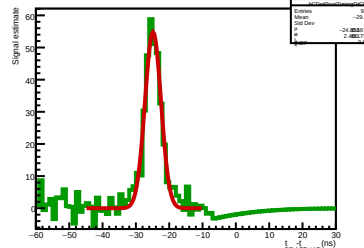
Background-subtracted, logical pixel ID 490
