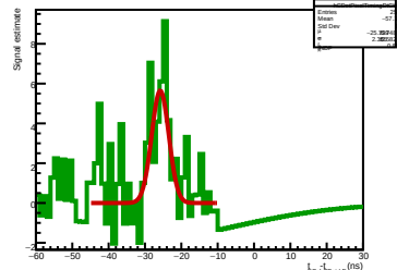
Background-subtracted, logical pixel ID 493
