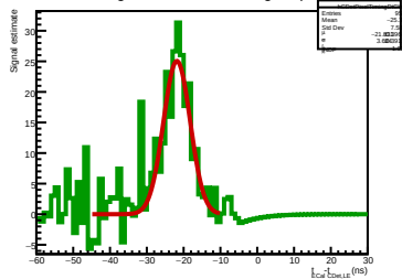
Background-subtracted, logical pixel ID 485
