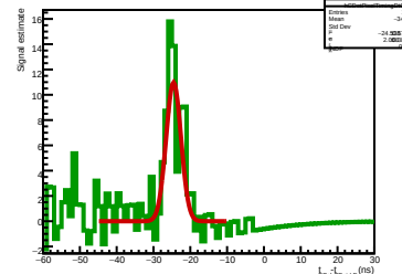
Background-subtracted, logical pixel ID 492
