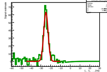
Background-subtracted, logical pixel ID 491
