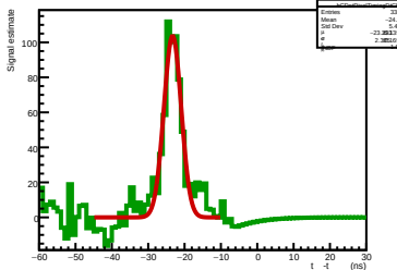
Background-subtracted, logical pixel ID 494
